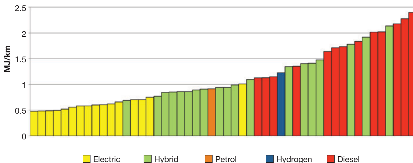
Figure 1: Energy consumption per vehicle
